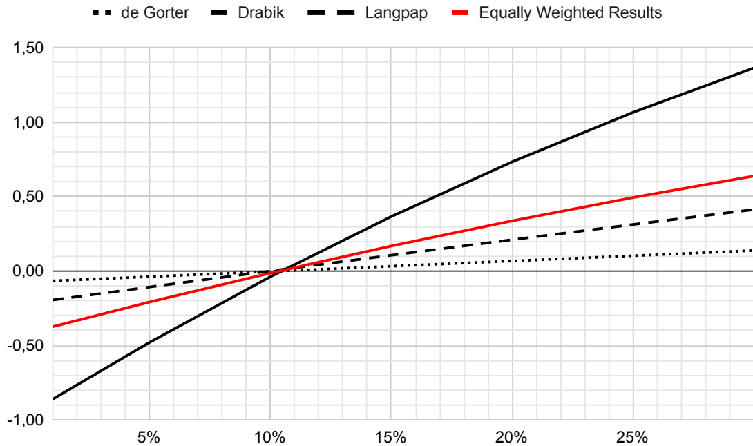
Figure 3: Projection of the savings resulting from different blend levels, averages of 2023-2030 in cents per gallon
