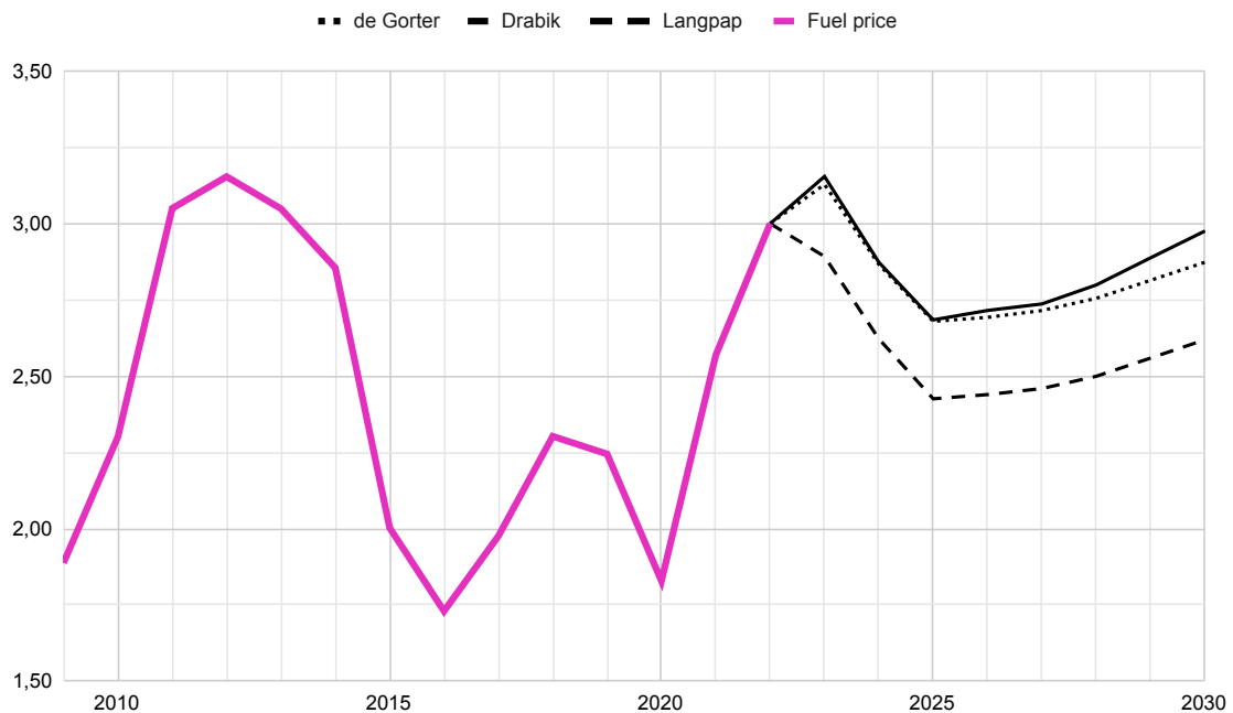
Figure 2: Projection of the fuel prices for 2023-2030
