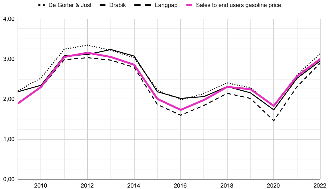
Figure 1: Comparison of simulated fuel prices obtained from the derived models and the actual sales to end users fuel price
