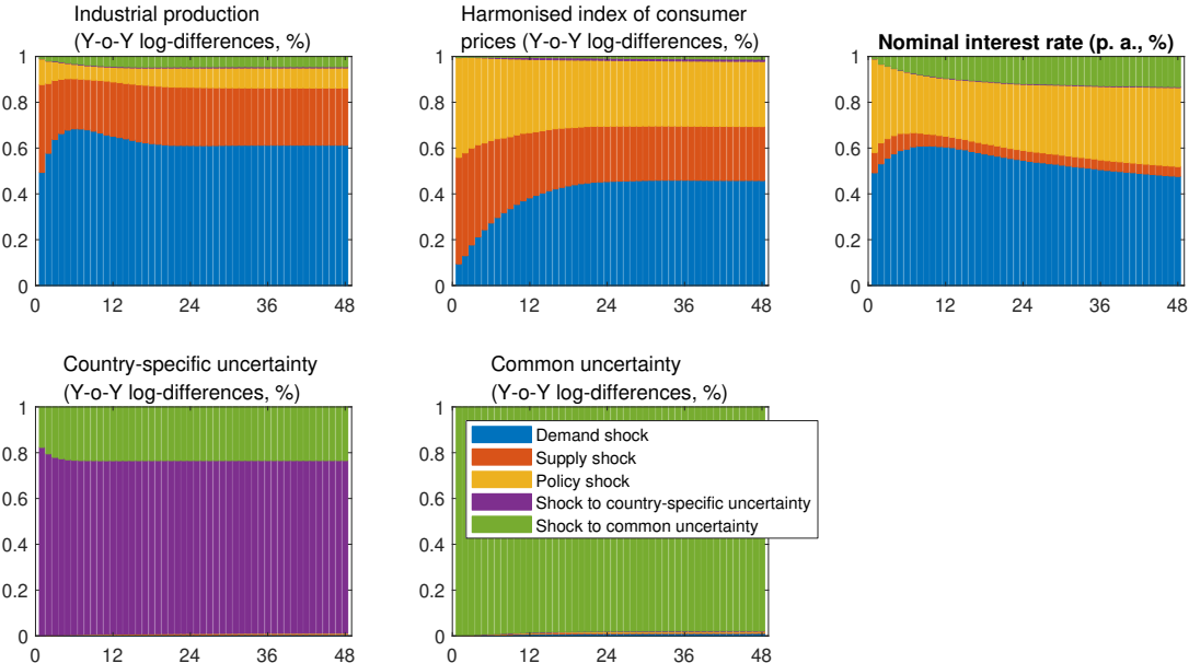
Figure 8: Forecast Error Variance Decomposition
