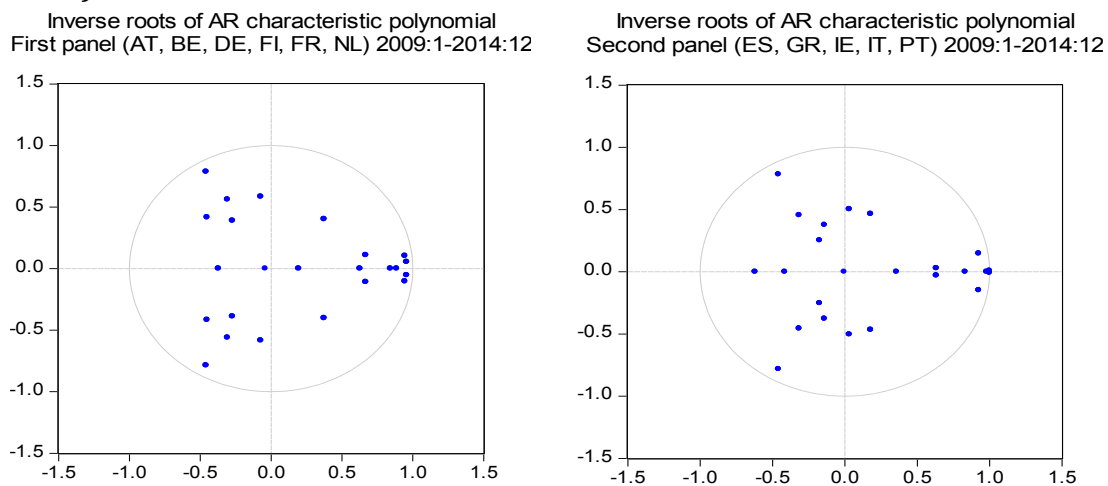
Chart A3: Inverse roots of the AR characteristic polynomial (2009:1-2014:12)
