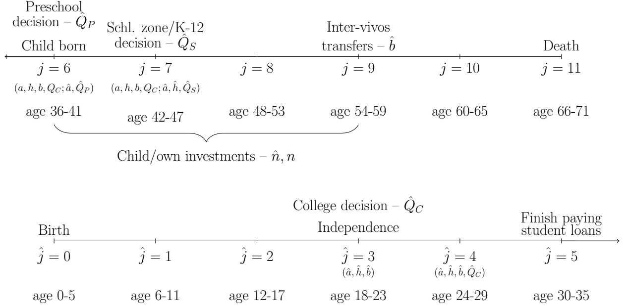
Figure 3: Lifecycle Timeline
