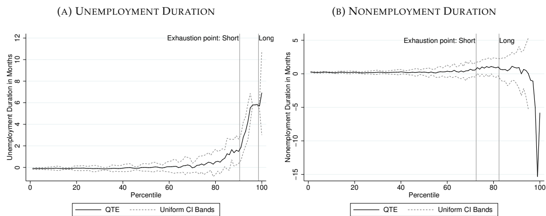
FIGURE S.1 QUANTILE TREATMENT EFFECTS ON DURATION AFTER PURGING THE RUNNING VARIABLE (AGE)
