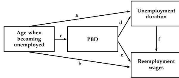
FIGURE 1 IV WITH TWO INTERDEPENDENT OUTCOMES
