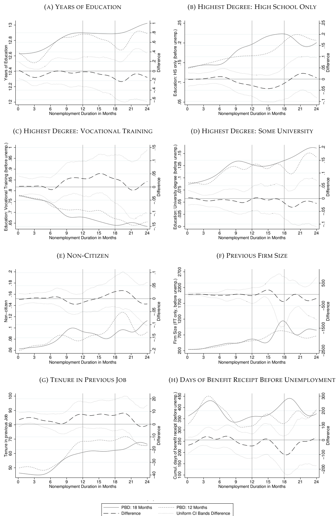
FIGURE S.10 DYNAMICS OF PRE-DETERMINED COVARIATES OVER THE NONEMPLOYMENT SPELL
