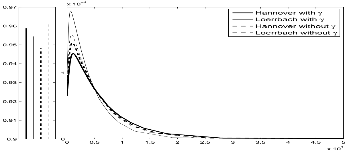
Figure 5: Estimated probabilities for zero total claim sizes (left panel) and density estimates of the positive total claim sizes (right panel) of the policyholders in the regions Hannover and L rrbach based on spatial (solid lines) and non spatial (dashed lines) models for both claim frequency and average claim size.
