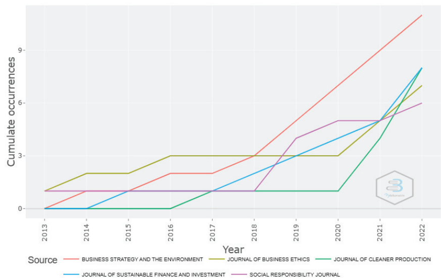
Figure 5. Source Growth.
