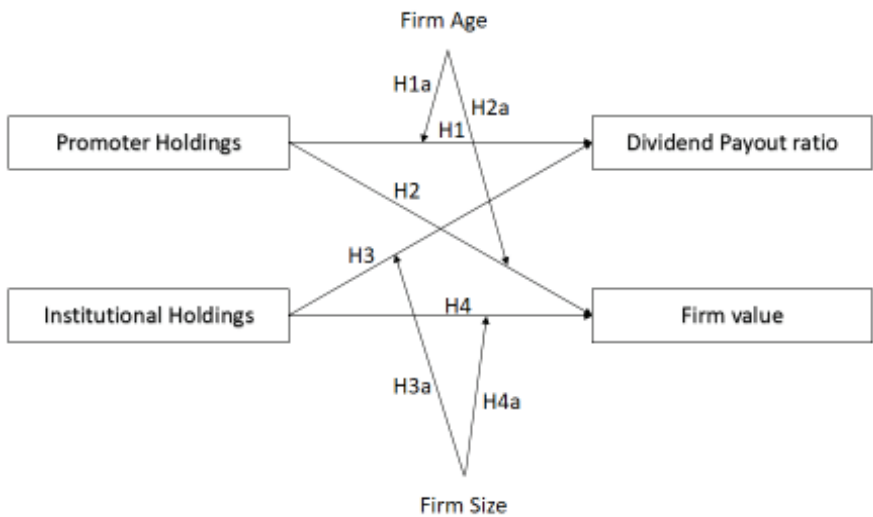
Figure 1. Conceptual Model.
