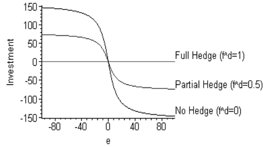
Figure 8: Investment function with f^d = 0 , f^d = 0.5 , and f^d = 1 .
