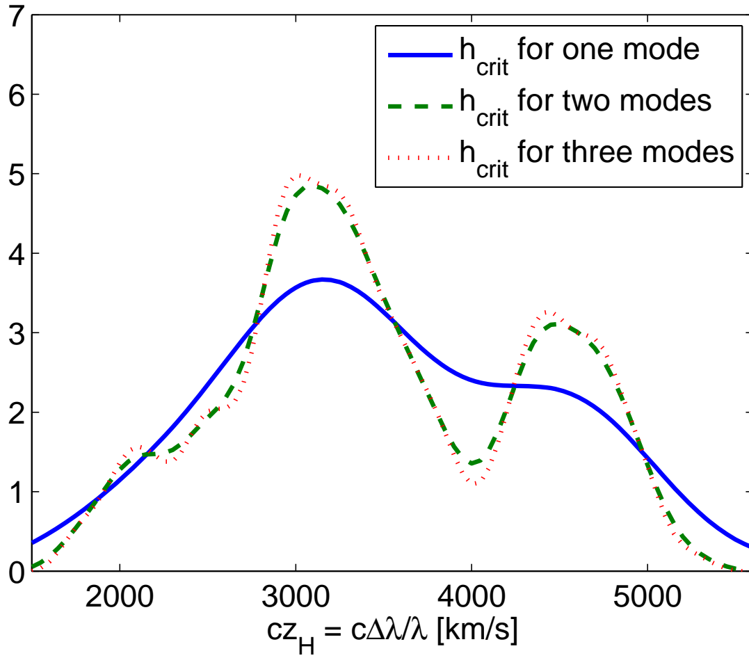
Figure 2: Estimates of the density of heliocentric escape velocities cz_H = c\Delta\lambda/\lambda [km/s] in the Centaurus cluster of galaxies corresponding to the critical bandwidth for one mode (solid line), two modes (dashed line) and three modes (dotted lines). See text for details.
