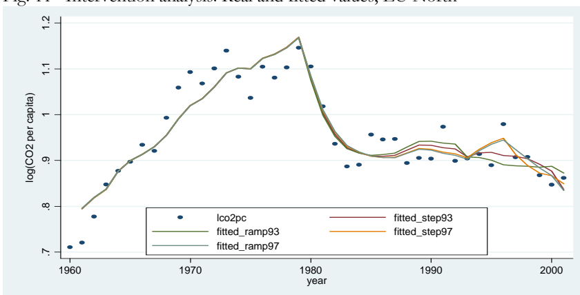
Fig. 11– Intervention analysis. Real and fitted values, EU North
