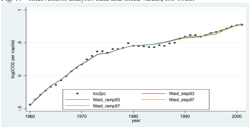
Fig. 10 - Intervention analysis. Real and fitted values, EU south
