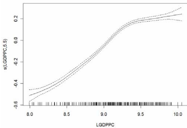
Figure 6 - GAM individual fixed effects (eq 8 with f(t) = 0 )
