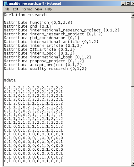
Figure 3: The quality_research.arff file
