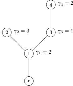
Fig. 1: Extended Tree with 4 players.
