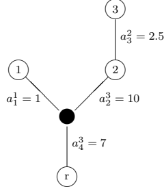
Fig. 3: Extended Tree in example 2.
