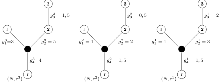
Fig. 4: Decomposition of the ET in example 2: player of type 1 boldface; player of type 0 normal type.
