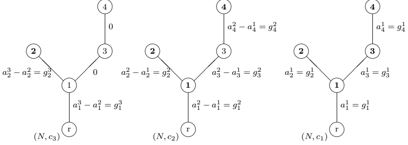
Fig. 2: Decomposition of the ET in Figure 1: player of type 1 boldface ; player of type 0 normal type.
