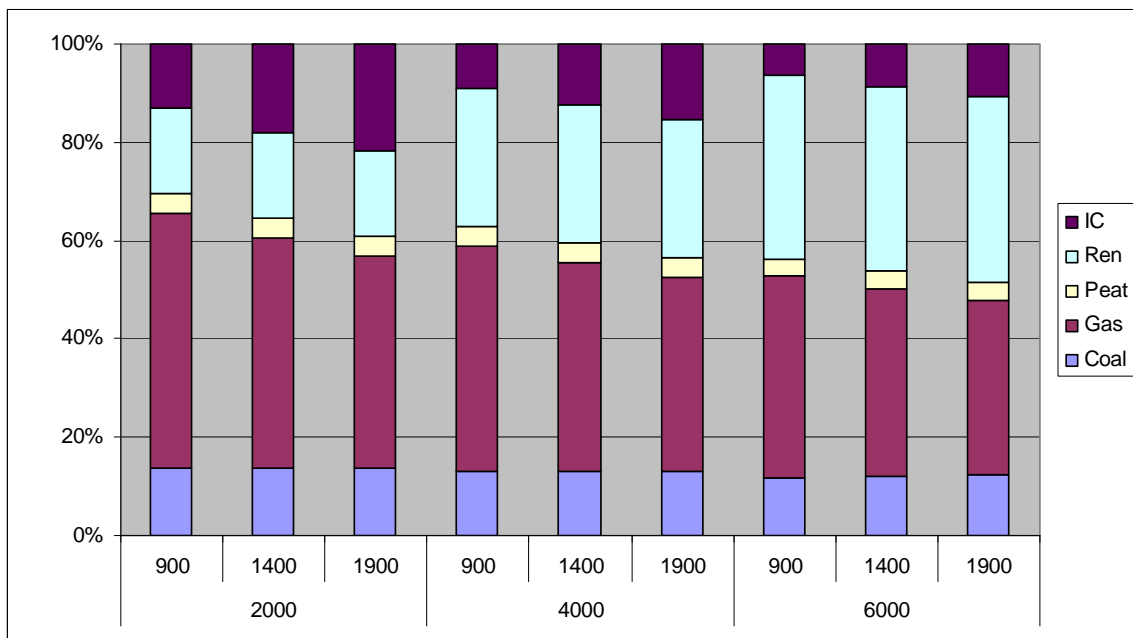
Figure 3. CCGT fuel shares in demand, medium fuel prices.
