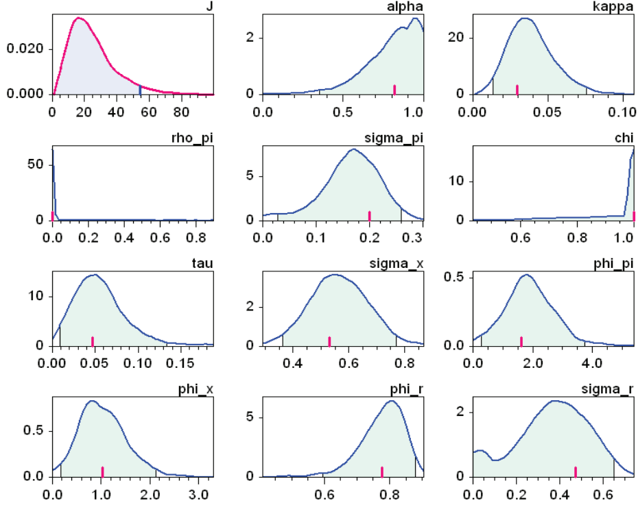
Figure 6: Frequency distributions of the re-estimations of the bootstrapped model A (GM).
