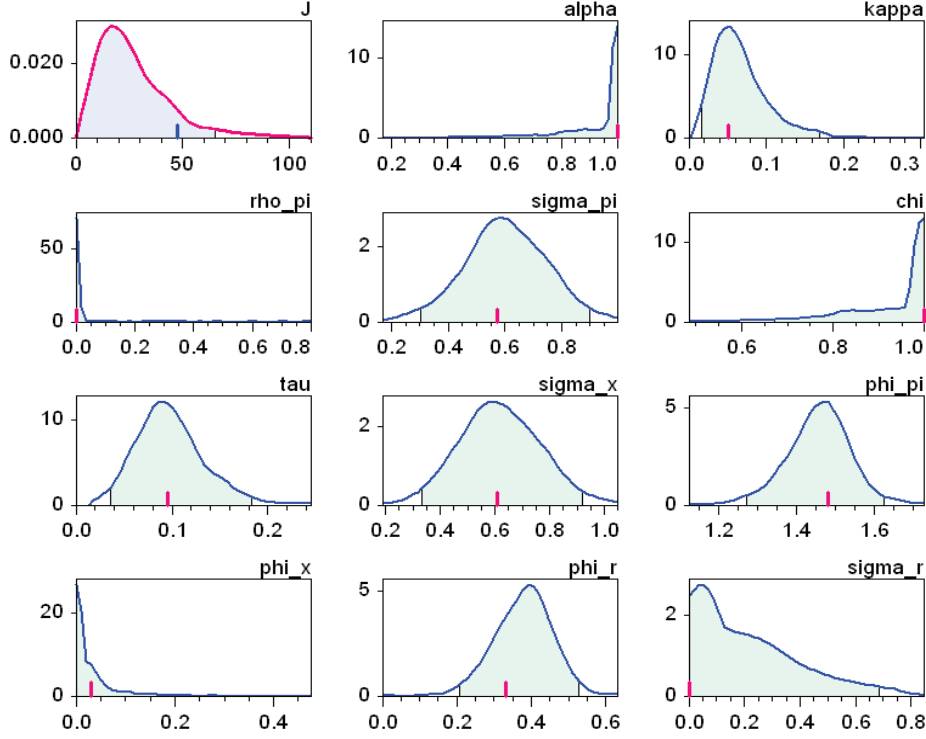
Figure 5: Frequency distributions of the re-estimations of the bootstrapped model A (GI).
