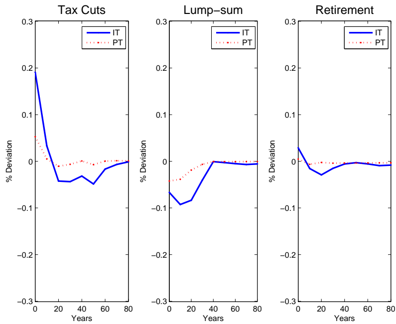
Figure 12: Output, 1% shock, for Different Policies under IT and PT, With Demographic Change
