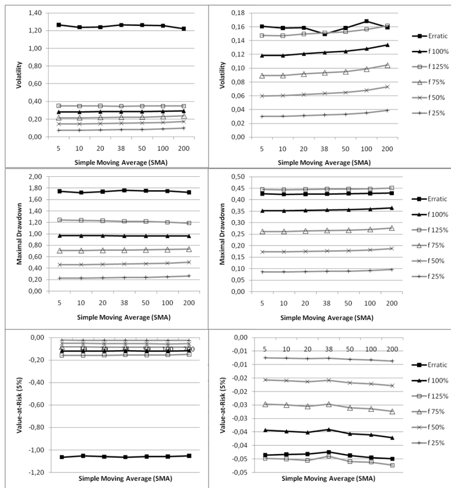
Figure 6: Risk figures dependent on volatility. The graphs show the volatility, the maximum drawdowns, and the value-at-risk (5%) for managed and unmanaged position sizing. On the left, the results for maximum volatility are displayed. On the right, the results for the minimum volatility are shown.
