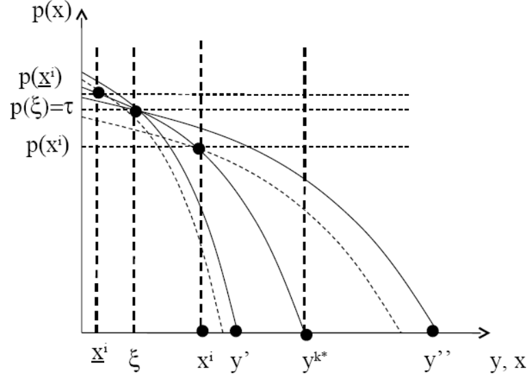
Figure 2: Security contours (solid) and indifference curves (dashed) for preferred reports for the case D > 0 in the proof of lemma 2.
