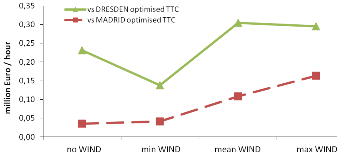
Figure 12: Total cost savings per hour using nodal pricing versus optimised TTC.
