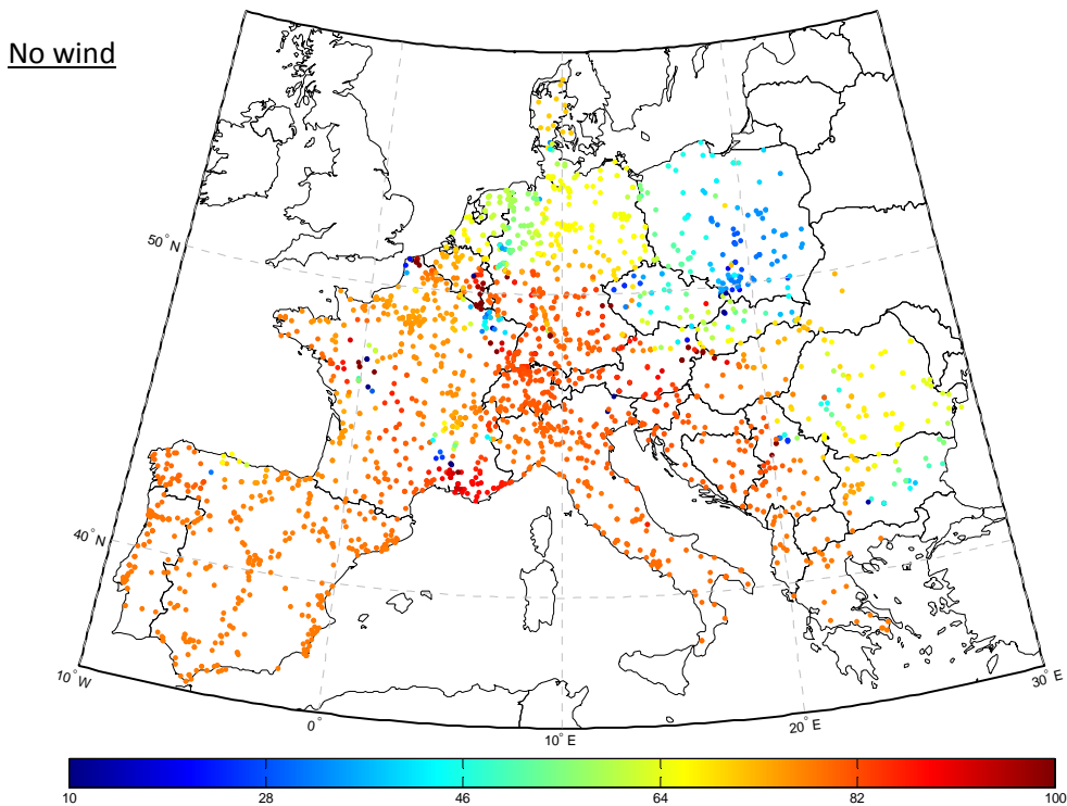
Figure 8: Geographic representation of nodal marginal prices. Bar represents energy prices at nodal level: from €10/MWh in blue to €100/MWh in red. (NO WIND scenario above, MAX below).
