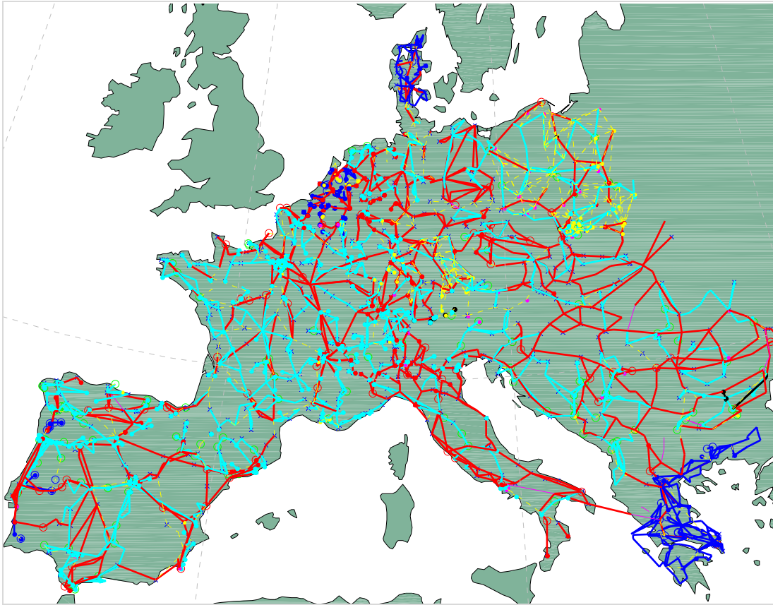
Figure 2: Network model geographic representation. Different line colours represent different voltage levels (red: 380kV, cyan: 220kV, blue: 150kV) and dotted lines correspond to equivalent elements.
