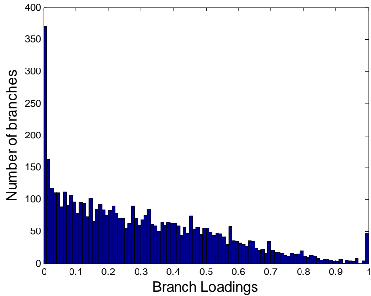
Figure 6: Distribution of branch loads (as a fraction of capacity) for the analysed high wind scenario.
