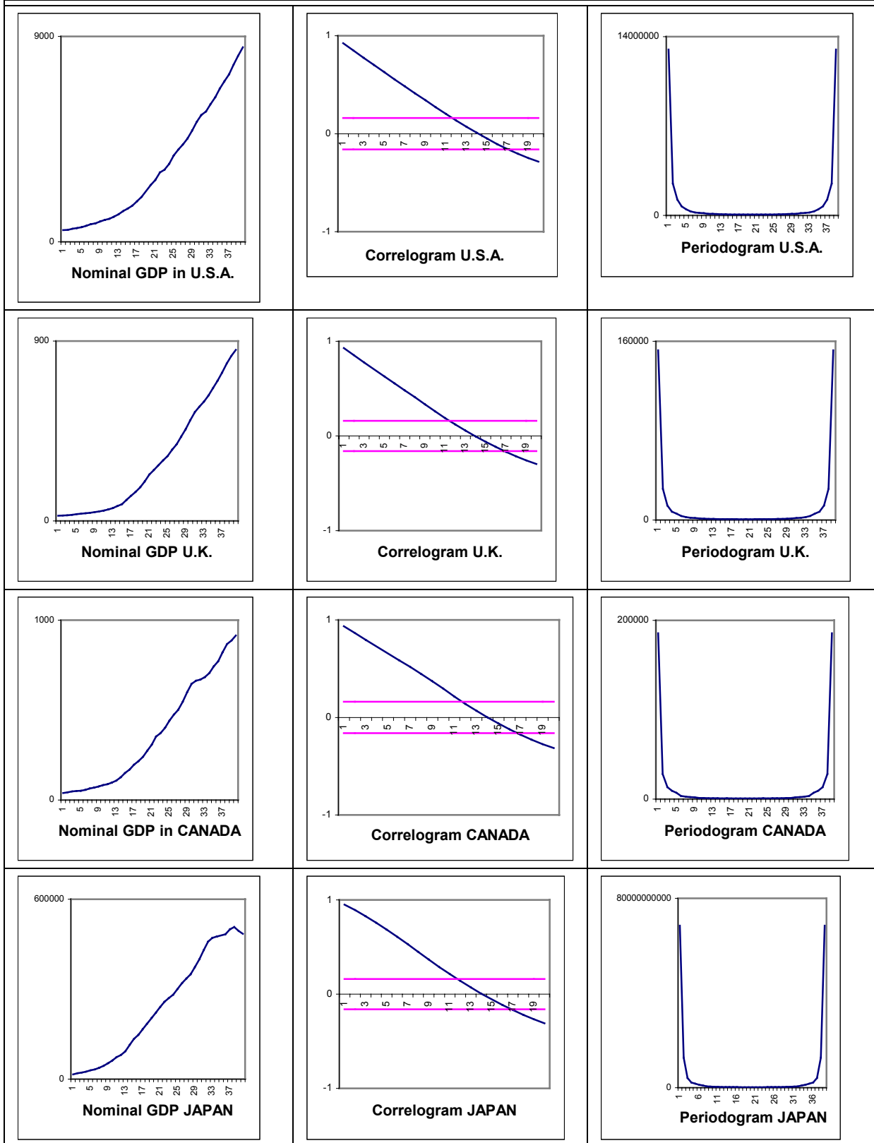
Original time series with their corresponding correlograms and periodograms
