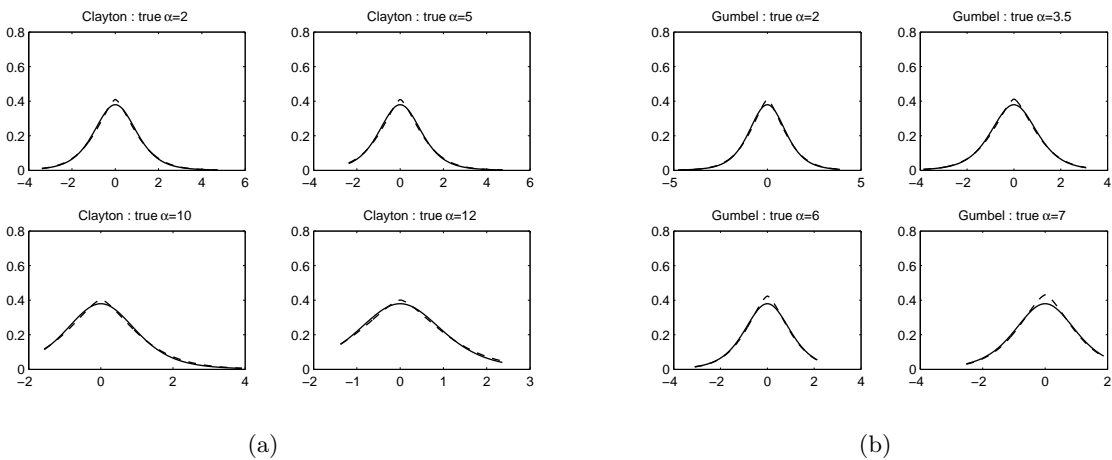
Figure 7: Sieve MLE of marginal density function for (a) Clayton copula, (b) Gumbel copula. True=solid, Sieve MLE=dashed. Evaluation is based on the common support of 1000 MC simulated data.
