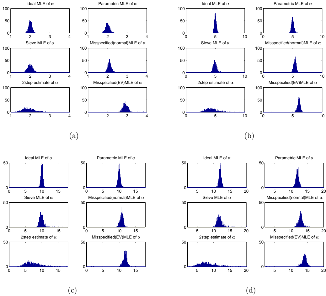
Figure 5: Clayton copula: Histograms of \alpha estimates (a)true \alpha=2 ,(b>true \alpha=5 , (c)true \alpha=10 , (d)true \alpha=12
