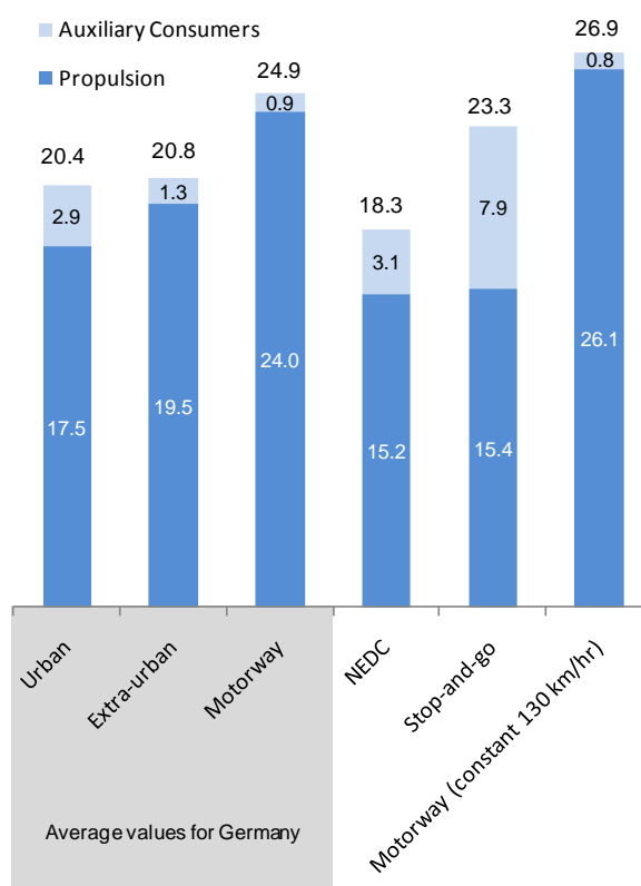
Figure 2: Modelled BEV Electricity Consumption for a Compact Car in Germany (kWh/100 km)
