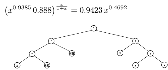
Figure 15: Best candidate frontier s_{\omega(1),5} in generation \mathcal{P}_5
