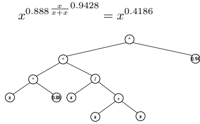
Figure 13: Best candidate frontier s_{\omega(1),3} in generation \mathcal{P}_3
