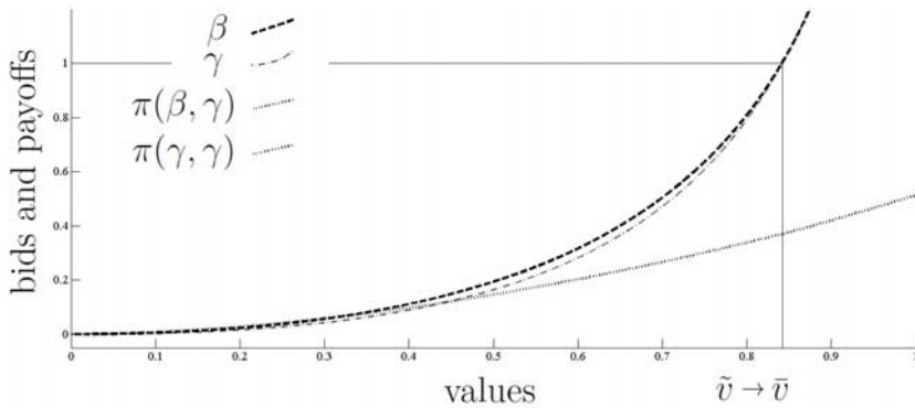
Figure 4: bids and payoffs for \theta = 1.1 .
