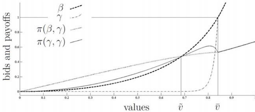
Figure 3: bids and payoffs for \theta = 10 .
