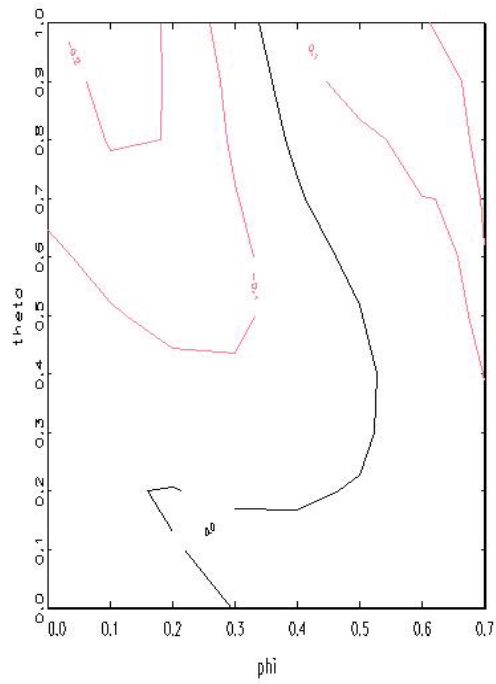
Figure 29: Difference of mean-absolute prediction error of MSE-DM-based model selection minus AIC-based model selection. Generating model is RC-ARMA( \phi, \theta ).
