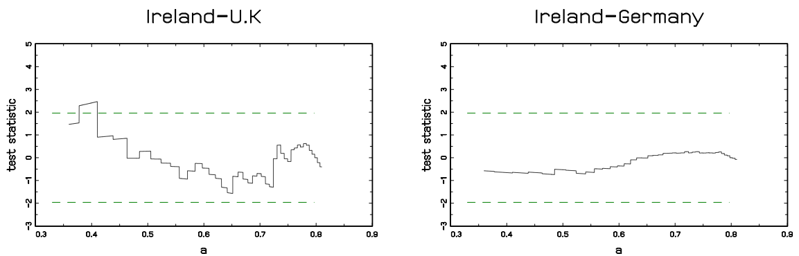
Figure 3: Perron-Qu t_d(a, 1; 0.8, 1) test
