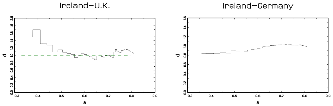
Figure 2: Estimate of d using GPH method with T^a frequencies
