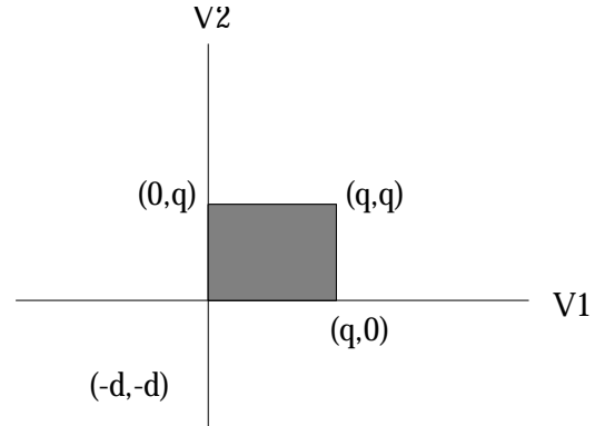
Figure 2: Stage-game payoffs
