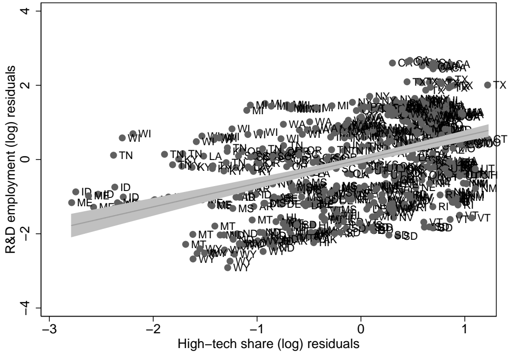
Figure 2: Outlier detection
