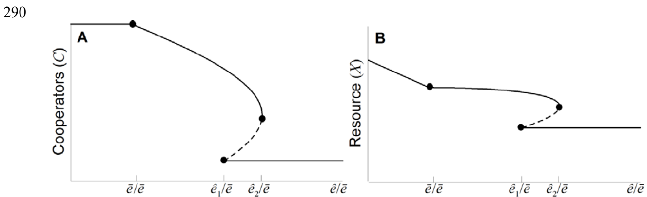
Figure 1. Bifurcation diagram showing internal equilibria of the number of cooperators C (panel A) and the resource stock X (panel B) for different values of \hat{e}/\bar{e} , reflecting the strength of the social dilemma. Stable equilibria are connected by solid lines, unstable equilibria are connected by dashed lines. Dots denote the two tipping points \hat{e}_1/\bar{e} and \hat{e}_2/\bar{e} , and the point \bar{e}/\bar{e}=1 , where the social dilemma materializes.
