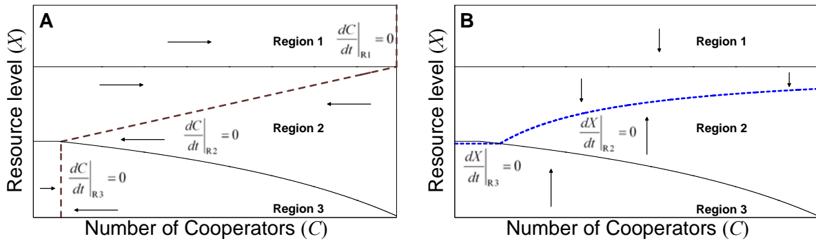
Figure 2. The nullclines (dashed lines) and direction vectors of the number of cooperators (panel A) and of the resource stock (panel B). The three different regions are separated by solid lines. 15
