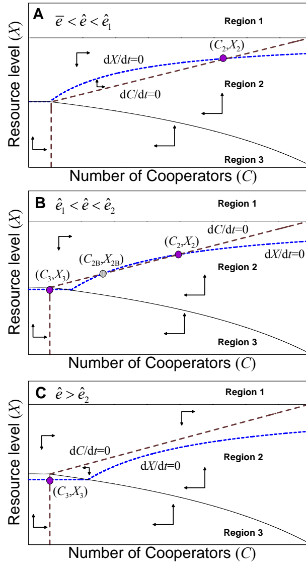
Figure 3. Phase planes showing the nullclines (dashed lines), the region boundaries (solid lines) and the vector fields for different values of \hat{e} . In panel A ( \bar{e} < \hat{e} < \hat{e}_1 ) and C ( \hat{e} > \hat{e}_2 ) there is only one stable equilibrium, while panel B ( \hat{e}_1 < \hat{e} < \hat{e}_2 ) exhibits alternative stable states. 16
