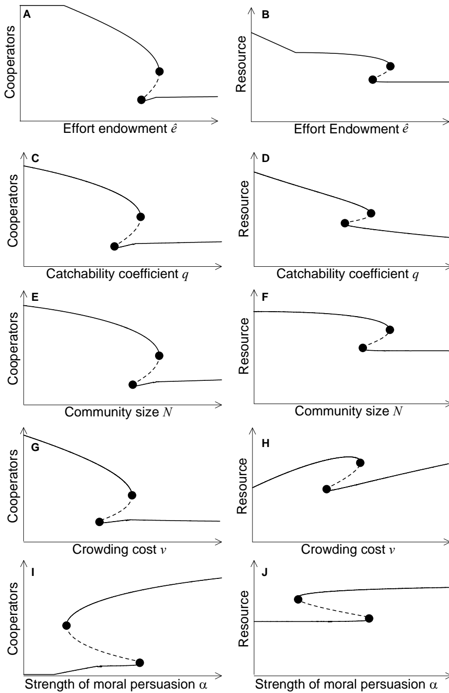
Figure 4. Bifurcation diagrams showing internal equilibria of the number of cooperators C and the resource stock X for w = 0.1 . Stable equilibria are connected by solid lines, unstable equilibria are connected by dashed lines, and dots denote the tipping points.
