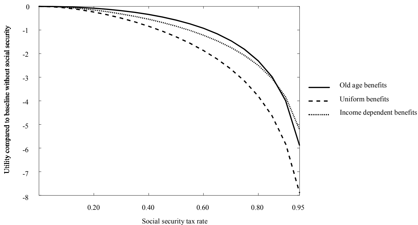
Figure 3. Social security and utility ( \alpha=0.5 ; \beta=0.5 )
