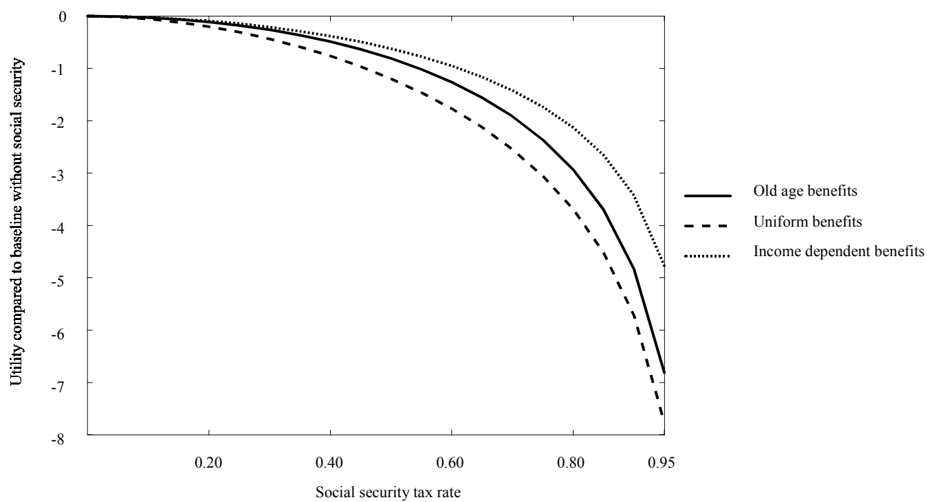
Figure 4. Social security and utility ( \alpha=0.5 ; \beta=1.5 )
