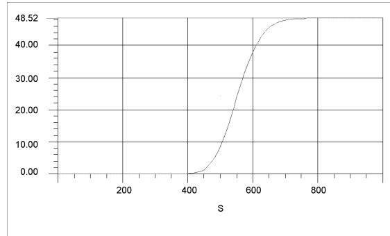
Figure 2: Premium of a Capped Symmetric Power Option
