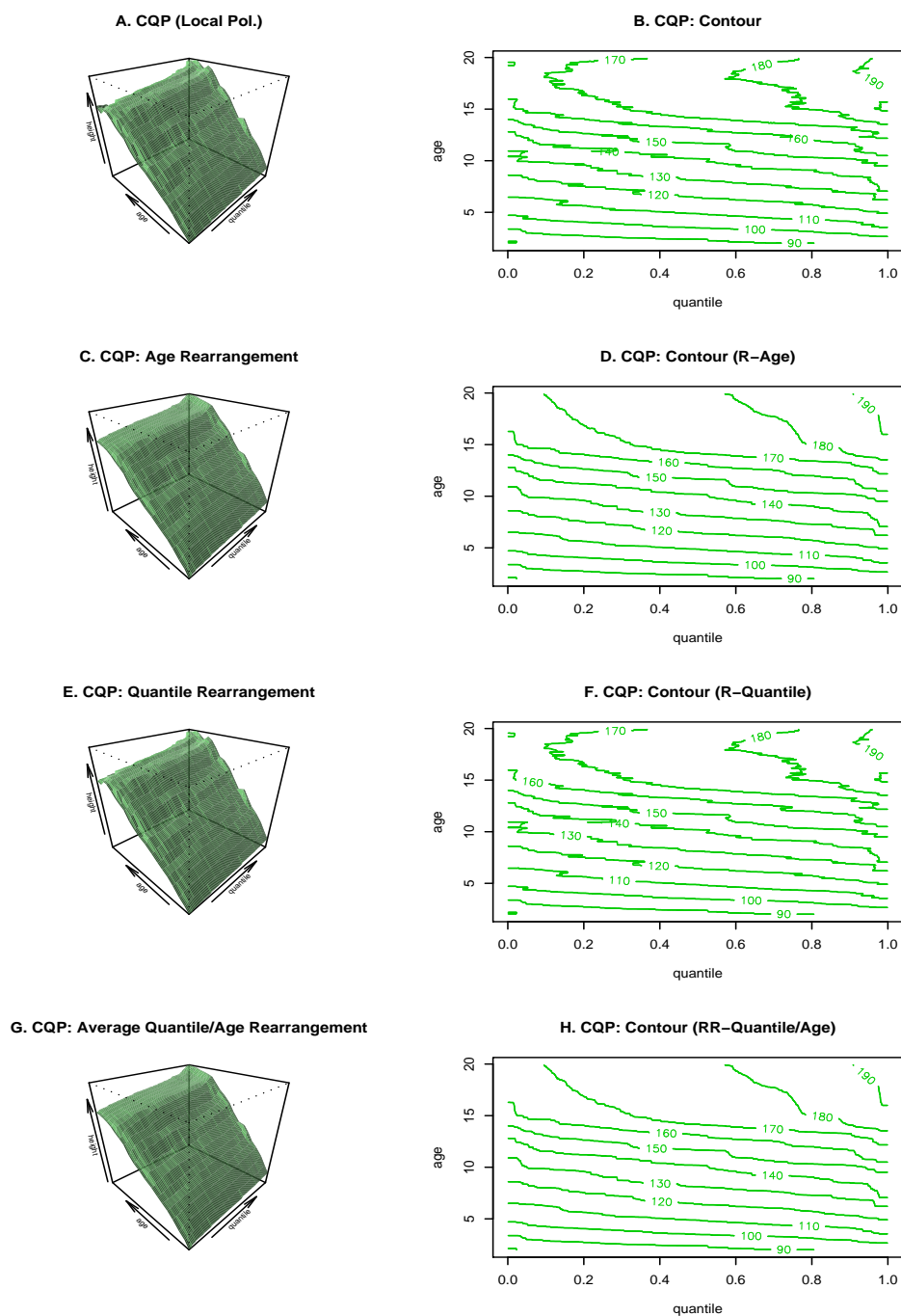
FIGURE 4. Locally linear estimates of the Conditional Quantile Process (CQP) of height given age and their increasing rearrangements. Panels C and E plot the one dimensional increasing rearrangement along the age and quantile dimension respectively; panel G shows the average multivariate rearrangement.
