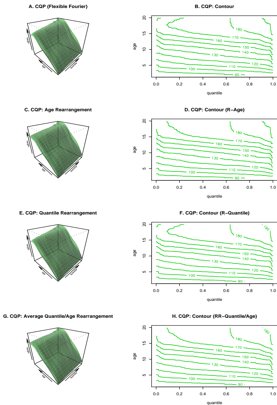
FIGURE 8. Flexible Fourier form series estimates of the Conditional Quantile Process (CQP) of height given age and their increasing rearrangements. Panels C and E plot the one dimensional increasing rearrangement along the age and quantile dimension respectively; panel G shows the average multivariate rearrangement.
