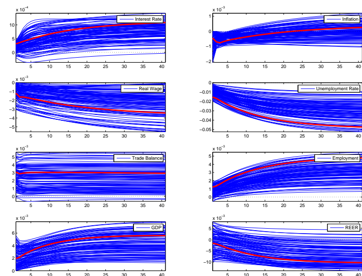
Figure 5: German impulse responses following a German wage markup shock
