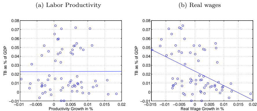
Figure 2: German productivity, real wages and the trade balance (1991Q2-2007Q4)
