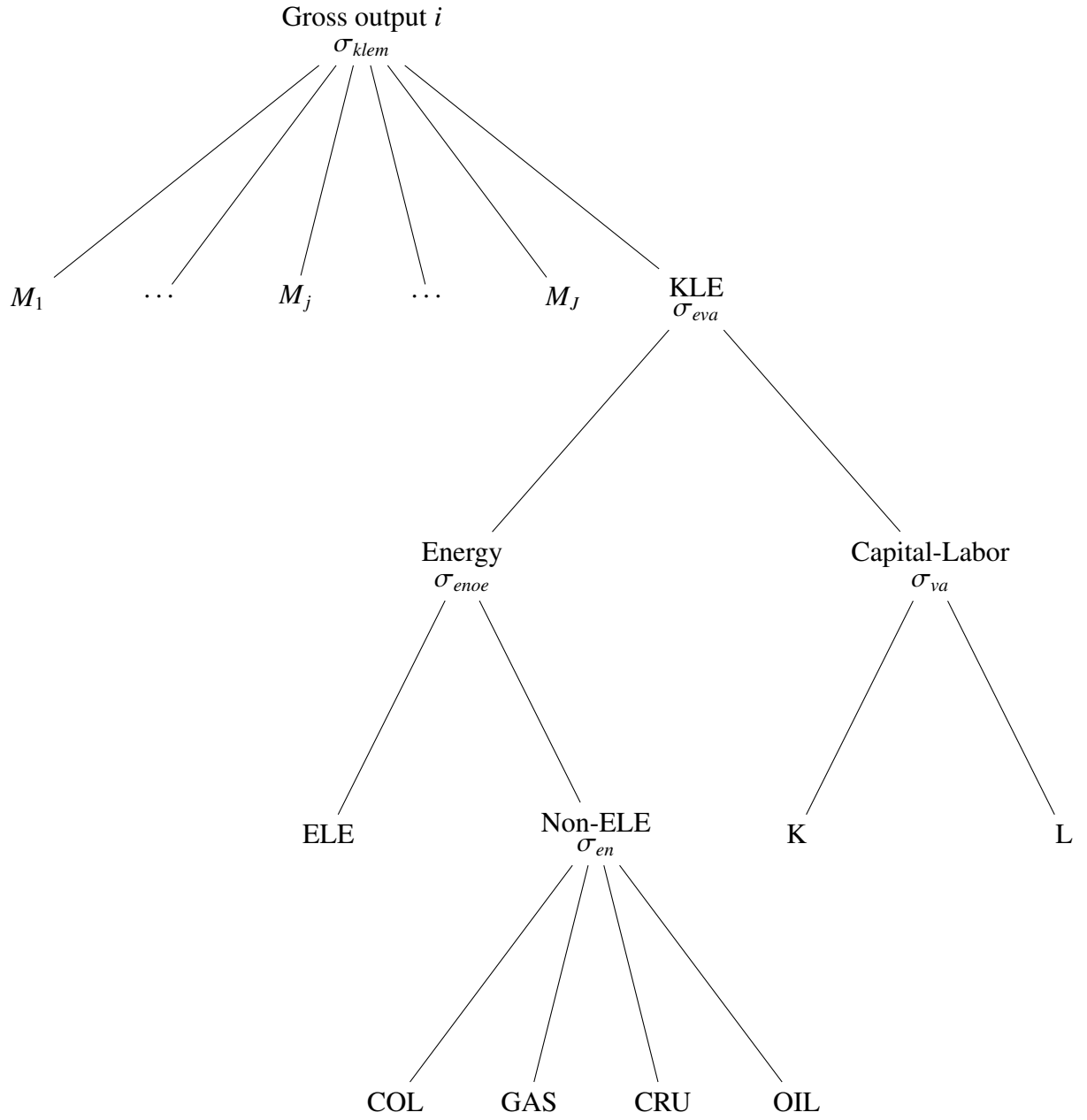
Figure A.10: Structure of production for i \in \{\text{TRN}, \text{EIS}, \text{SRV}, \text{CRP}, \text{LS}, \text{NFM}, \text{NMM}, \text{PPP}, \text{MAN}\} .
