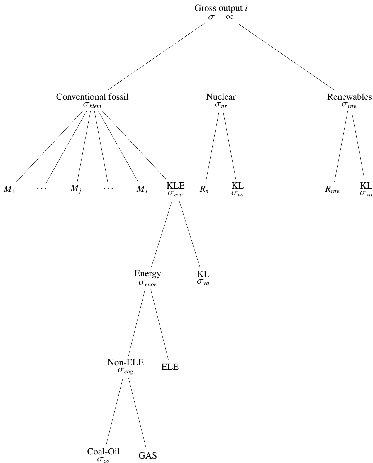
Figure A.14: Structure of electricity production i \in \{ELE\} .
