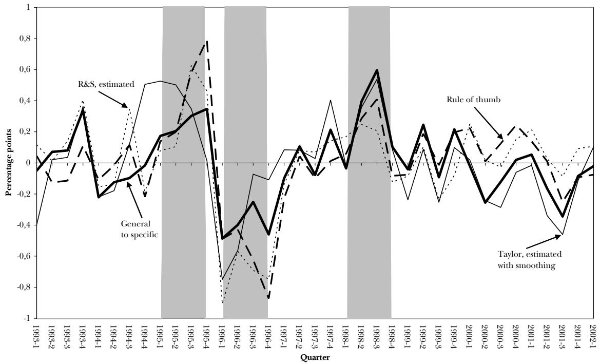
Fig. 2: Policy deviations (residuals) from estimated simple rules
