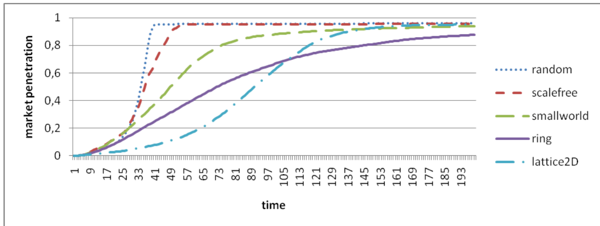
FIGURE 1 Diffusion curves for different network topologies
