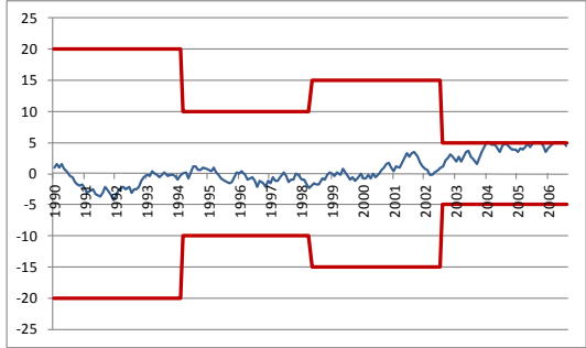
Figure 2: No-arbitrage band unidentifiable (example)
