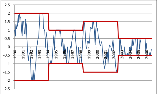
Figure 1: Relative prices in the band of no-arbitrage (example)
