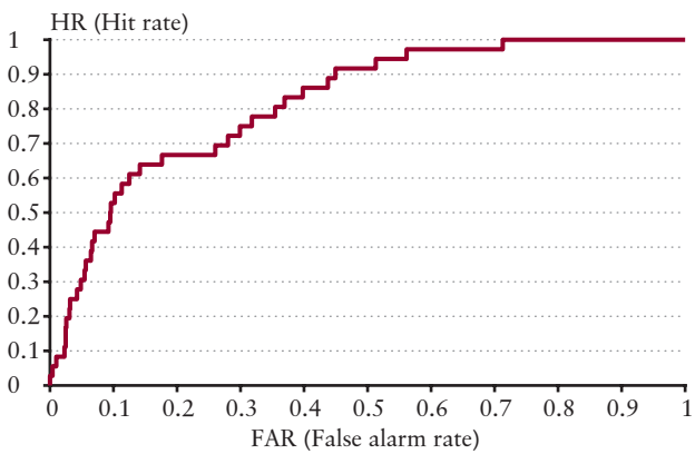
ROC curve of the first neural network model (Network 1)
