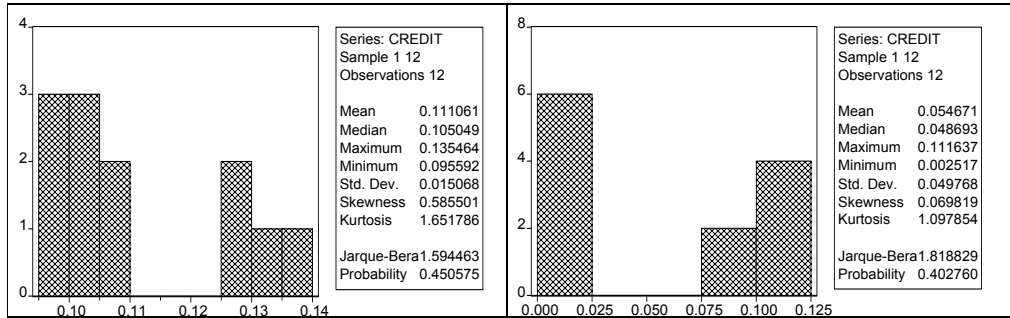
Figure 5. Distribution of the Variance Decompositions of the Credit Shock, with 1st and 2nd Orderings.
