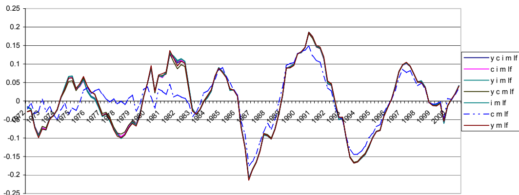
Figure 4. The Credit Shock under Alternative Identifications
