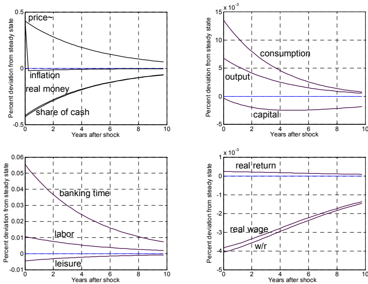
Figure 1. Impulse responses to 1 % credit productivity shock
