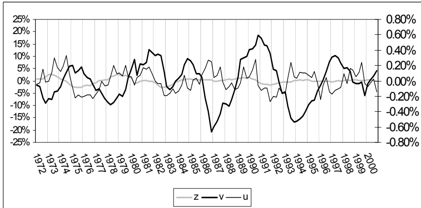
Figure 2. Evolution of productivity ( z ), credit ( v ) and money ( u ) shocks ( u on the right axis)
