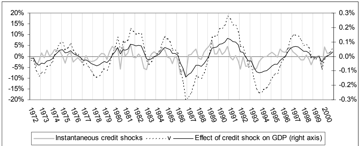
Figure 3. Credit innovations ( \hat{\epsilon}_{vt} ), the credit shock ( v_t ), and the effect of credit shocks on GDP ( \frac{GDP_{actual}}{GDP|_{v=0}} - 1 )
