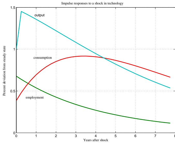
Figure 10: Impulse Responses (Model-I), \Phi = 0.5
