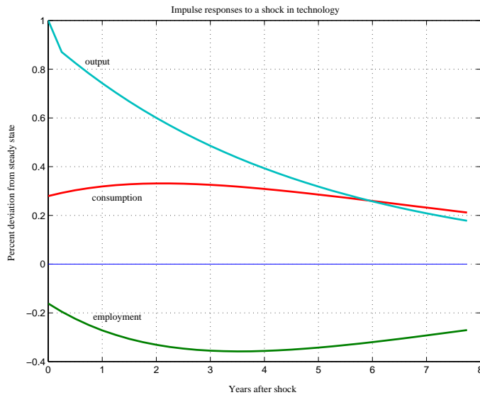
Figure 11: Impulse Responses (Model-I), \Phi = 2.0
