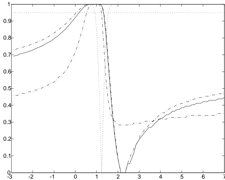
Figure 6: p -value plots of statistics that test the hypothesis H_0 : \beta = \beta_0 for dataset with \pi_1 = 0.1 , k = 5 . statistic (18) (-), Anderson-Rubin (- -), LR (-.-), 2sls t -statistic (..).
