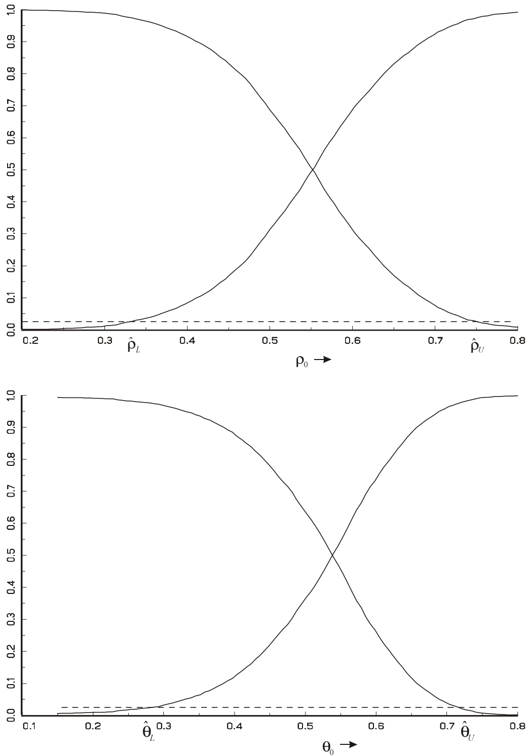
Figure 3: Bootstrapped p -values based on the test statistic approach for the null hypotheses H_0: \rho = \rho_0 and H_0: \theta = \theta_0 against their one-sided alternatives ( B = 4999 ).
