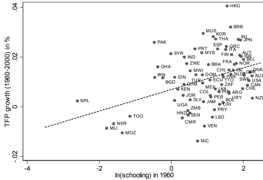
Figure 2: Scatterplot of TFP growth (1960-2000) against \ln(\text{schooling}) in 1960
