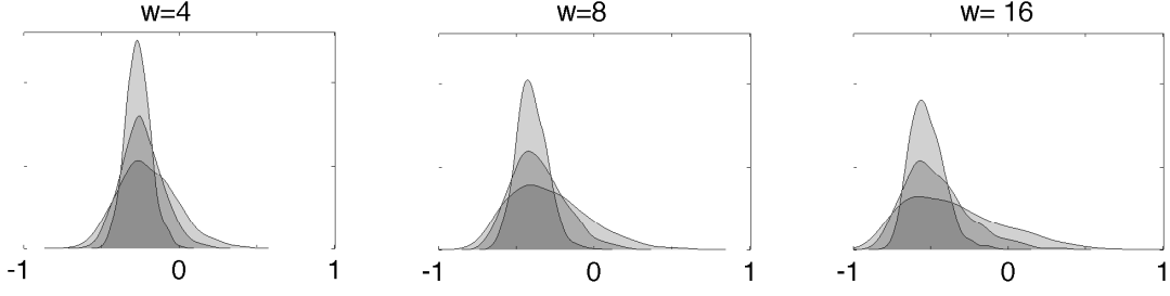
Figure 4: Density plots of \hat{\rho}_T^{w,s,z} obtained from S = 1000 Monte Carlo simulated paths of \{(y_t, x_t, z_t)\}_{t=1}^T under phase-dependence ( \beta = -0.3 ), for window size w = 4 (left), w = 8 (center) and w = 16 (right), and sample size T = 100, 250 and 500 . The larger T densities are identifiable by the smaller variance.
