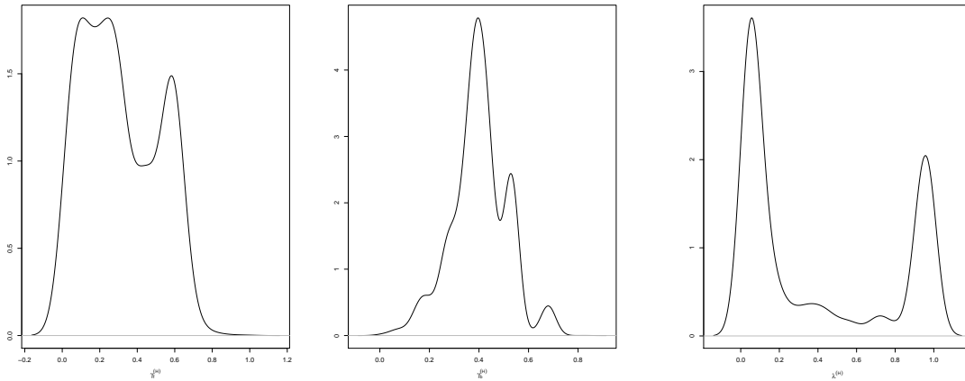
Figure 14: Posterior density of \lambda^{(H)} , \gamma_b^{(H)} and \gamma_f^{(H)} from the HPCS-TV model
