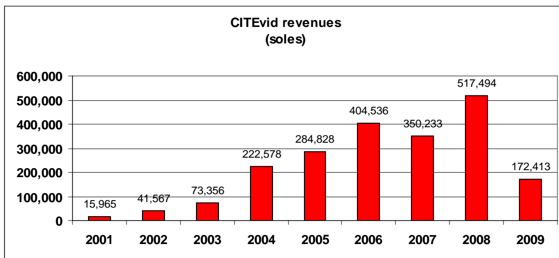
Figure 6. CITEvid Revenues
