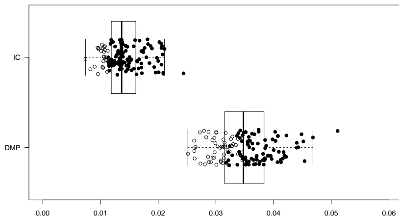
Figure 2: Variation of the coefficient on IC (model RE III) and DMP (model RE DMP) for all 136 possible subsets of 15 out of 17 regions. Box-plots and individual values shown. Solid dots indicate statistical significance at the 0.05 level.
