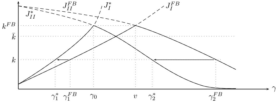
Figure 2: Distortions in information acquisition
