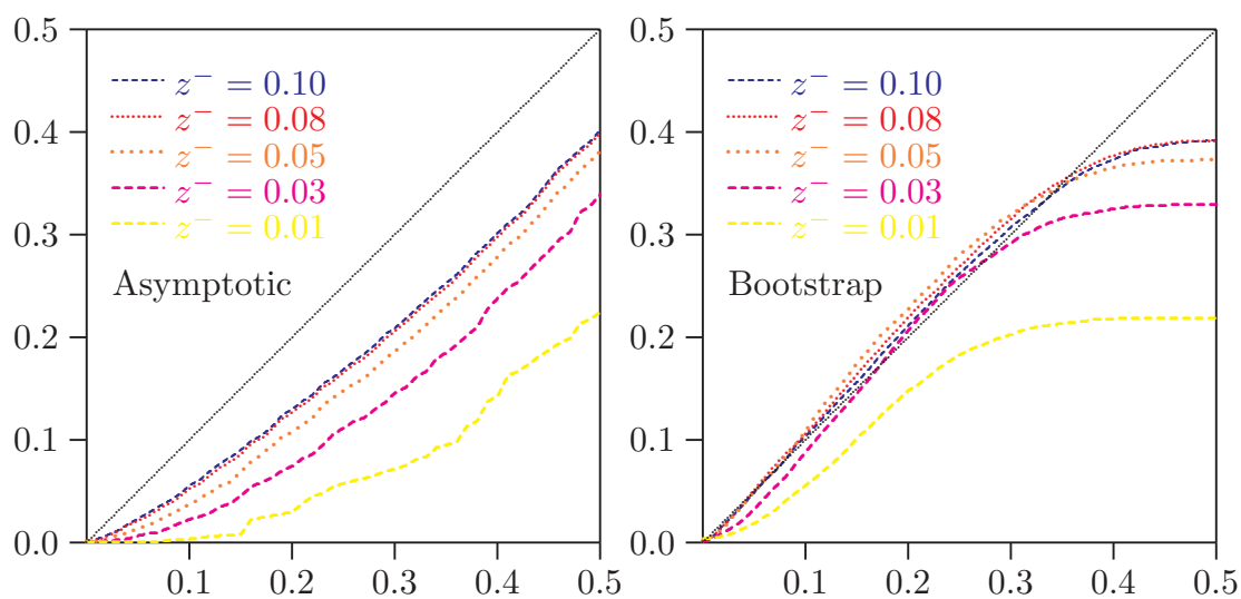
Figure 3: Varying amounts of discretisation; base case, N_A = 128
