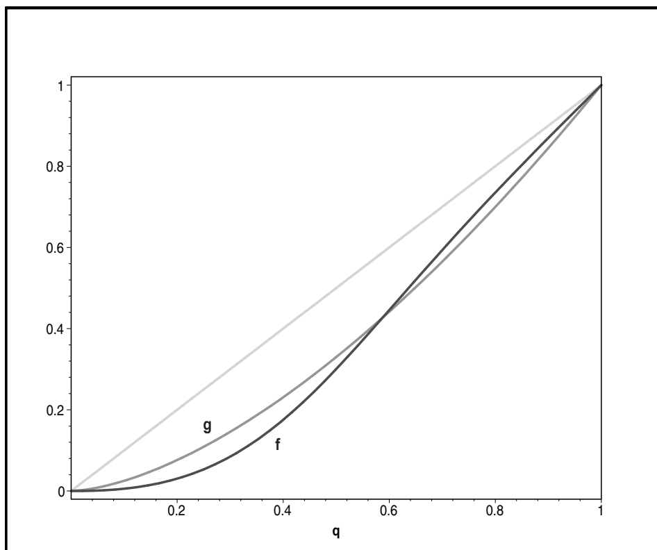
Figure 4.2: Star-Shaped and Convex Weighting Functions
