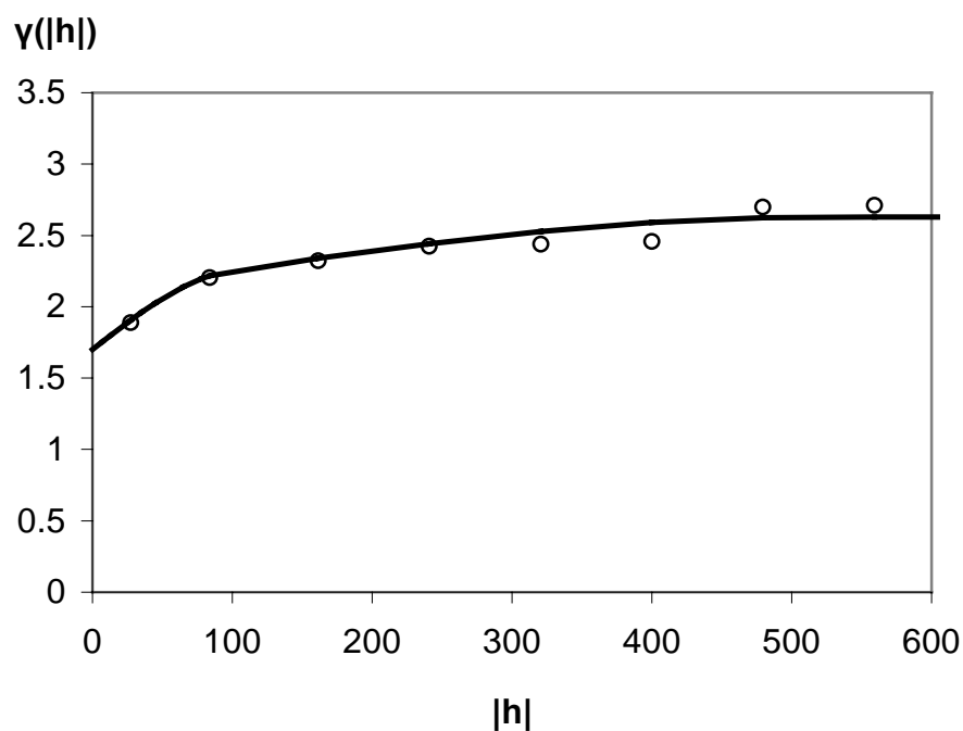
Figure 4: empirical variogram (dots) and modelled nested spherical variogram (line) for plot-wise time trend; |h| = distance in km; nugget: 1.7, sill1: 0.4, range1: 97.2 km, sill2: 0.53, range2: 520 km.
